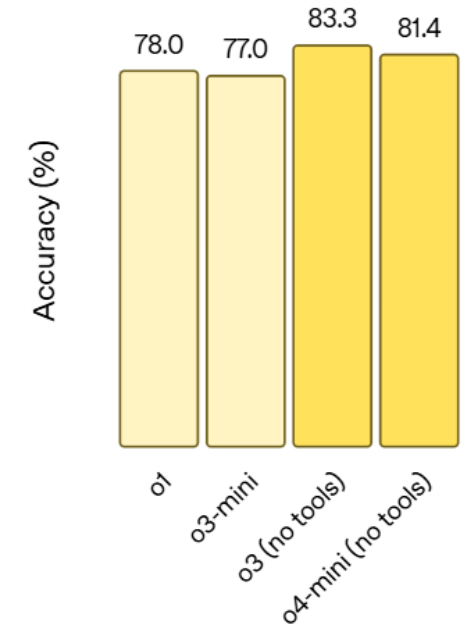
GPQA Diamond PhD-Level Science Questions
