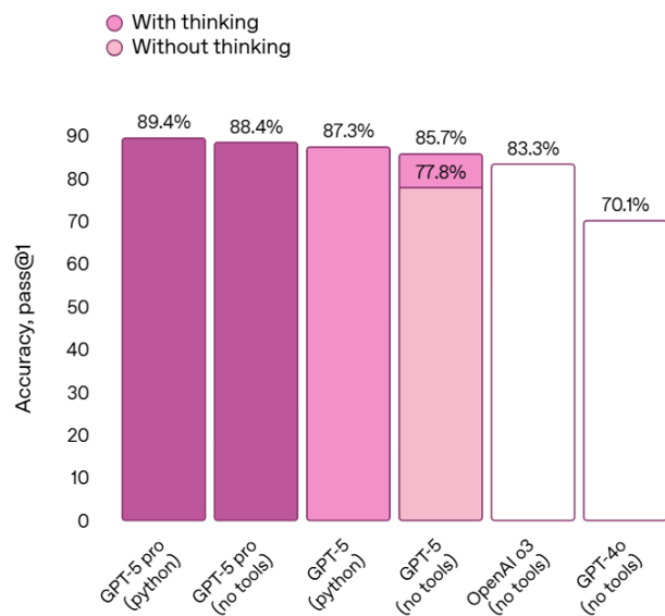
PhD-level science questions
